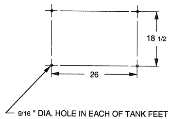
TANK FEET HOLE PATTERN
