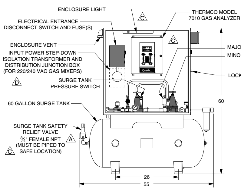
FRONT VIEW (DOOR REMOVED)
