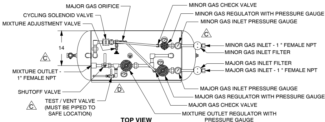
TOP VIEW (TOP REMOVED, GAS ANALYZER AND HORN NOT SHOWN)
